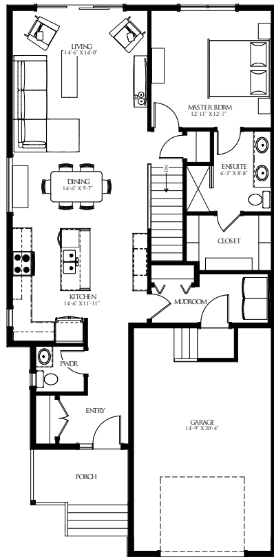
MAIN FLOOR PLAN LIVING AREA: 1,107 SQ FT
