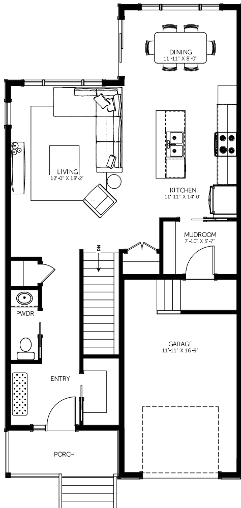
MAIN FLOOR PLAN LIVING AREA: 783 SQ_FT
